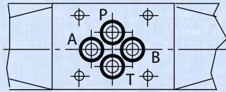
Mounting surface to ISO 4401 size 3
