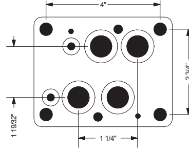
D07 Used on: DG5S4 04 DG5V 7 DG3V 7 4WEH16 4WH16
